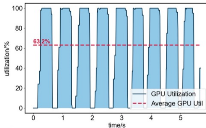
ZeRO-Offload
