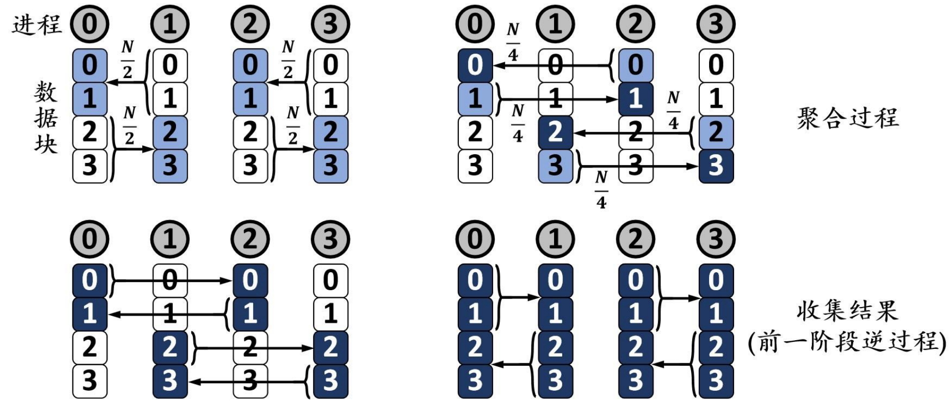
Rabenseifner Algorithm (an enhanced naïve halving-doubling)
